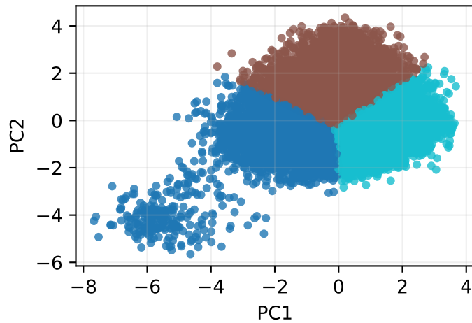
K-Means
