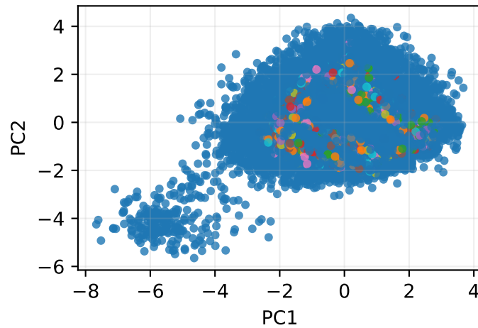
DBSCAN
