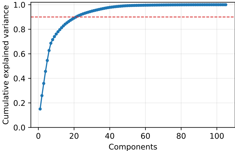
PCA scree: Adult Income
