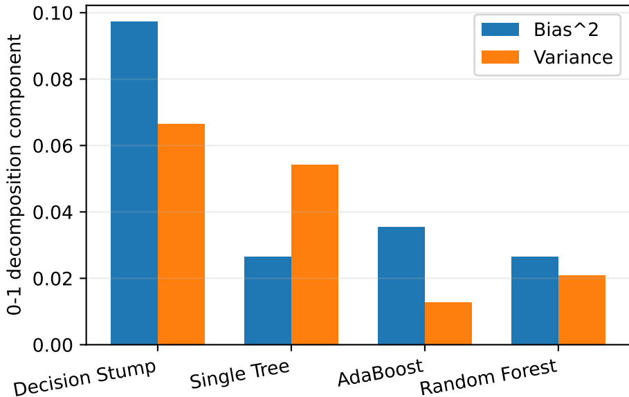
Bias-variance on Breast Cancer Wisconsin
