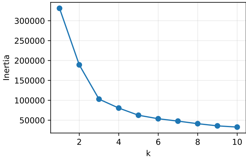
K-Means elbow: Covertypes
