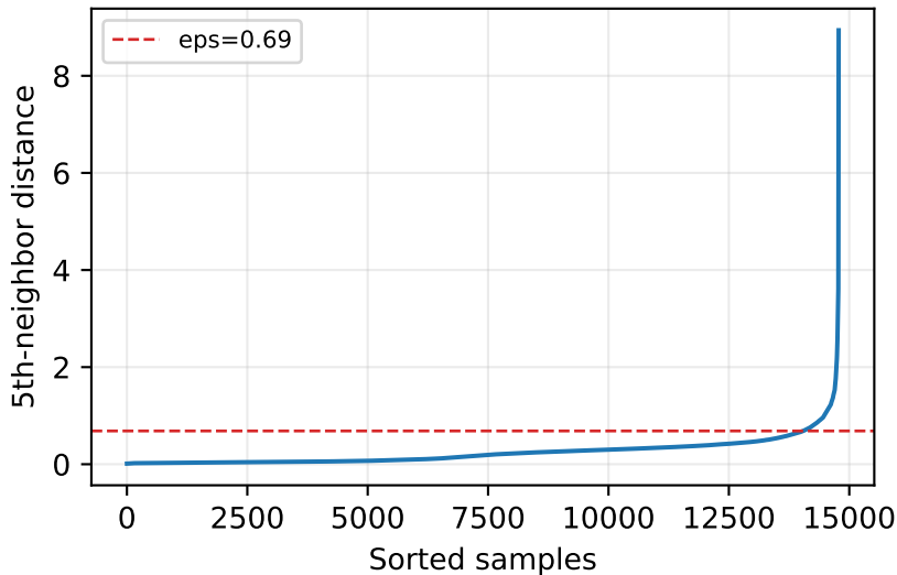
DBSCAN k-distance: MNIST2Class
