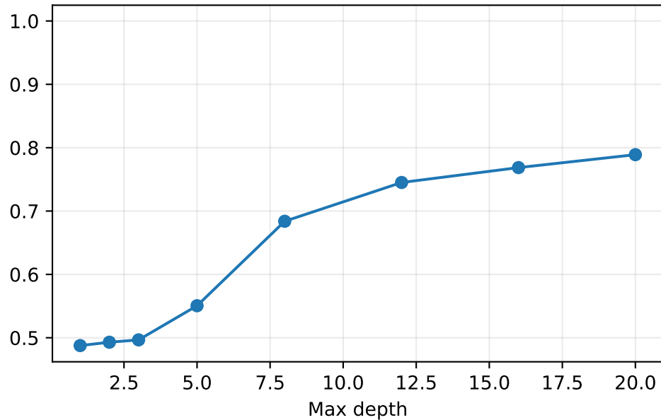
Covertypes
