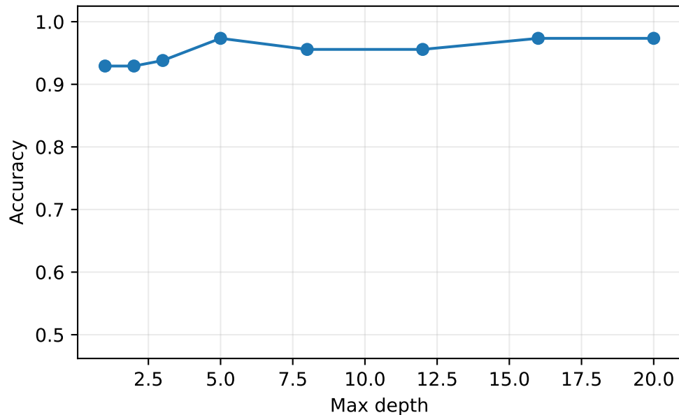
Covertypes
