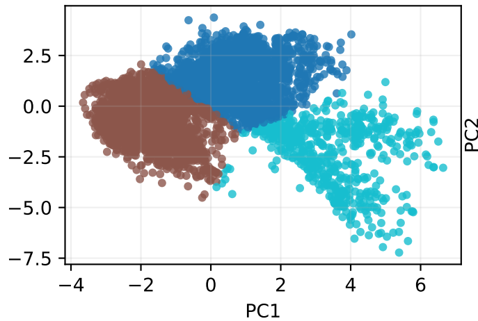
K-Means
