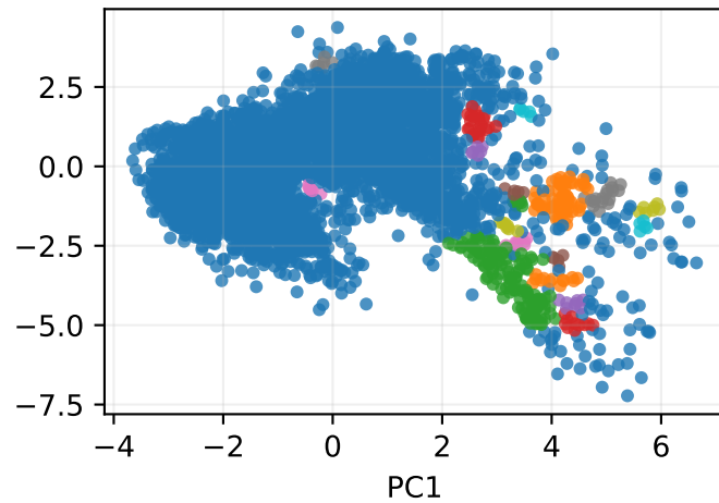
DBSCAN
