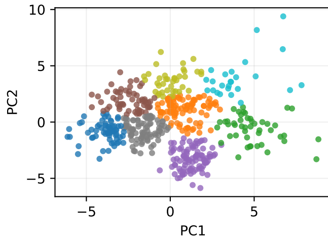
K-Means
