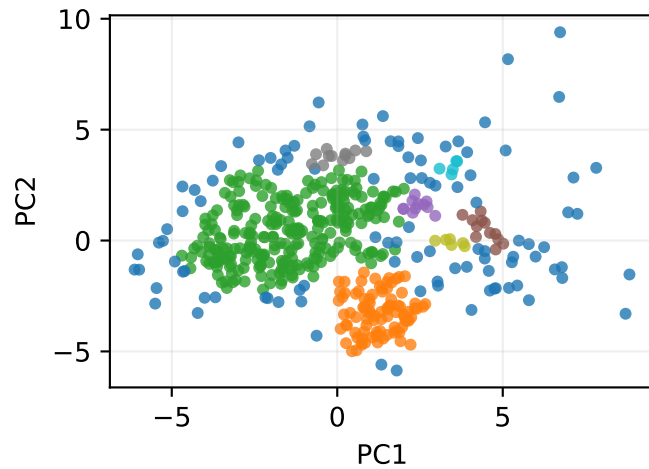
DBSCAN
