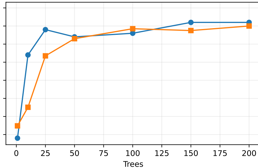
Digits High-Dimensional
