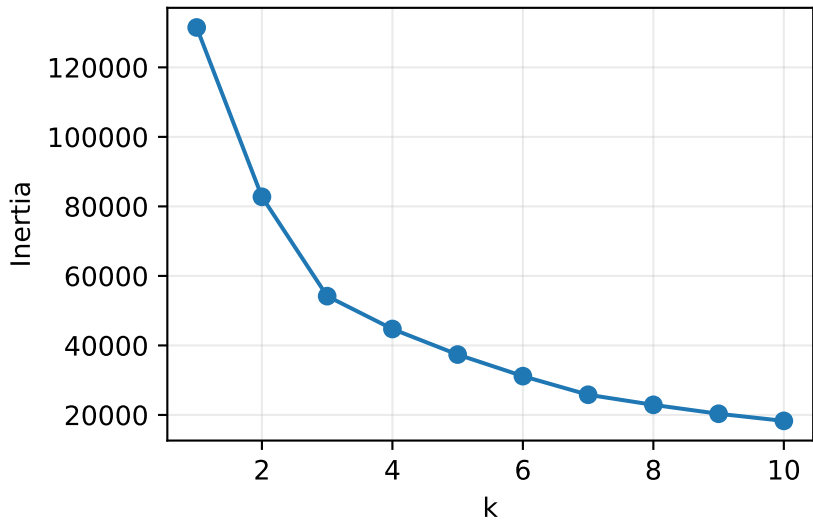
K-Means elbow: Adult Income
