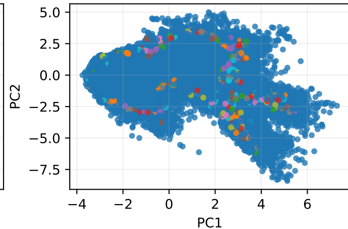
DBSCAN
