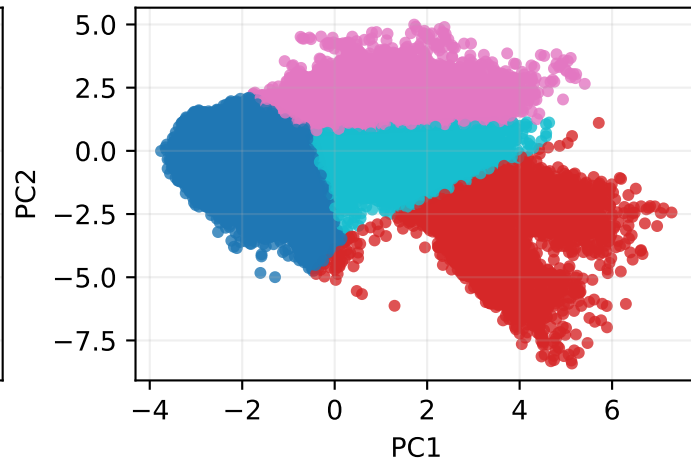
K-Means
