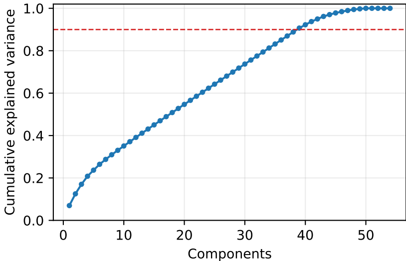
PCA scree: Covertypes
