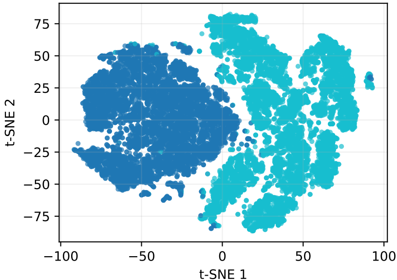
t-SNE bonus: MNIST2Class (all 14,780 rows)
