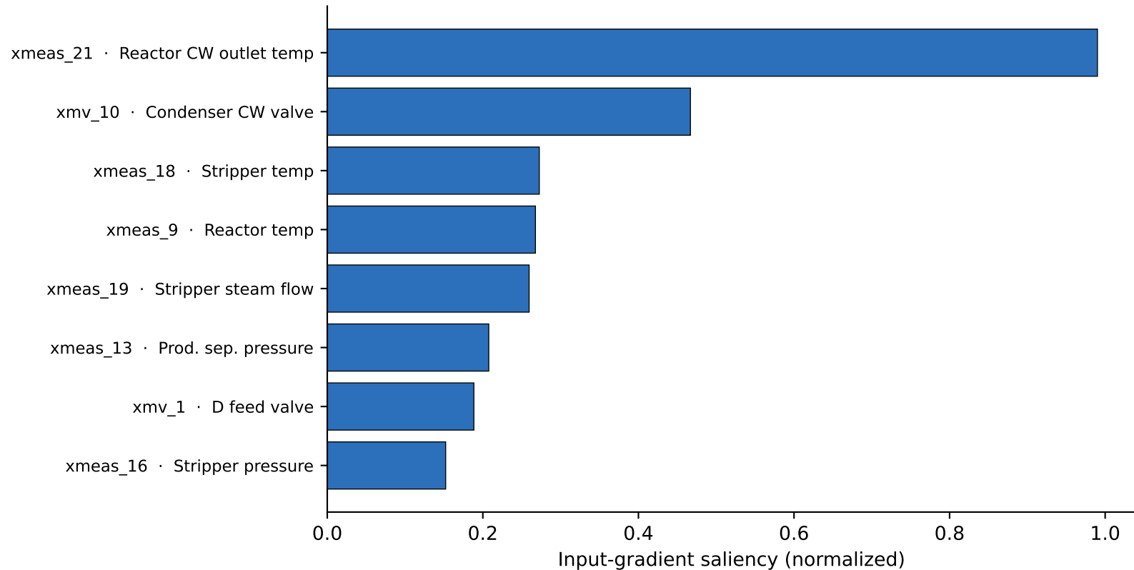
Figure 4. Variable attribution on Tennessee Eastman
