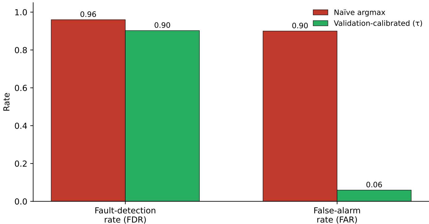
Figure 5. Calibrated threshold fixes the false-alarm problem (mean detection delay 47.8 min)
