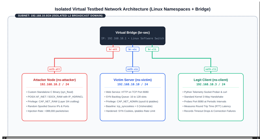
Figure 3.1: Architectural Block Diagram of the Isolated Virtual Testbed Network.
