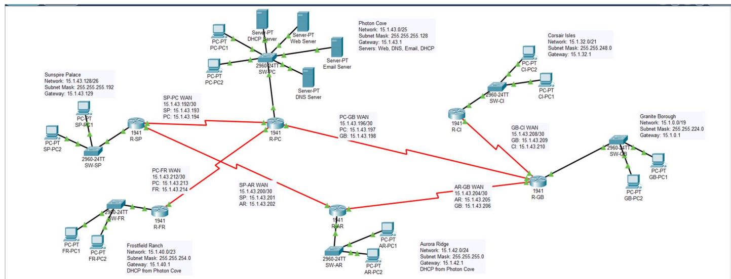
Figure 1: Final Topology Diagram with Network Notes
