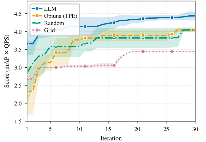
Figure 4: Best Score ( \text{mAP} \times \text{QPS} ) vs. iteration on HICO-DET (mean \pm 1\sigma , 3 seeds; 2 runs for Grid). LLM reaches \text{Score} \approx 3.97 at iteration 6; Optuna TPE at iteration 27, Random Search at iteration 28.
