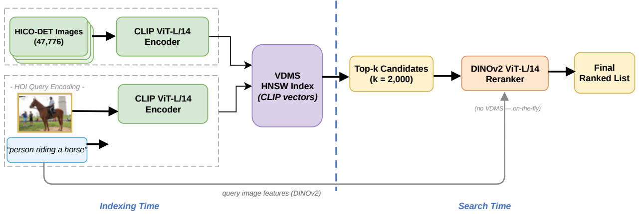
Figure 1: Two-stage retrieval pipeline (oracle O(\theta) ). Stage 1: CLIP ViT-L/14 ANN retrieval produces a top-k candidate pool. Stage 2: DINOv2 ViT-L/14-reg4 distances are fused via convex combination s_j = (1-\alpha)\hat{c}_j + \alpha\hat{d}_j , re-ranking candidates at zero additional indexing cost. Score = mAP \times QPS.
