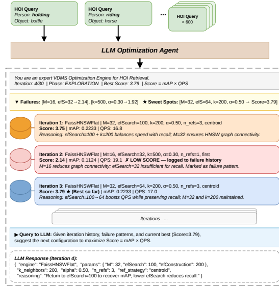
Figure 3: LLM prompt structure. The system prompt encodes parameter physics; the user prompt supplies g(\mathcal{H}_{t-1}) , history, and untried-value hints, eliciting a structured JSON configuration response.
