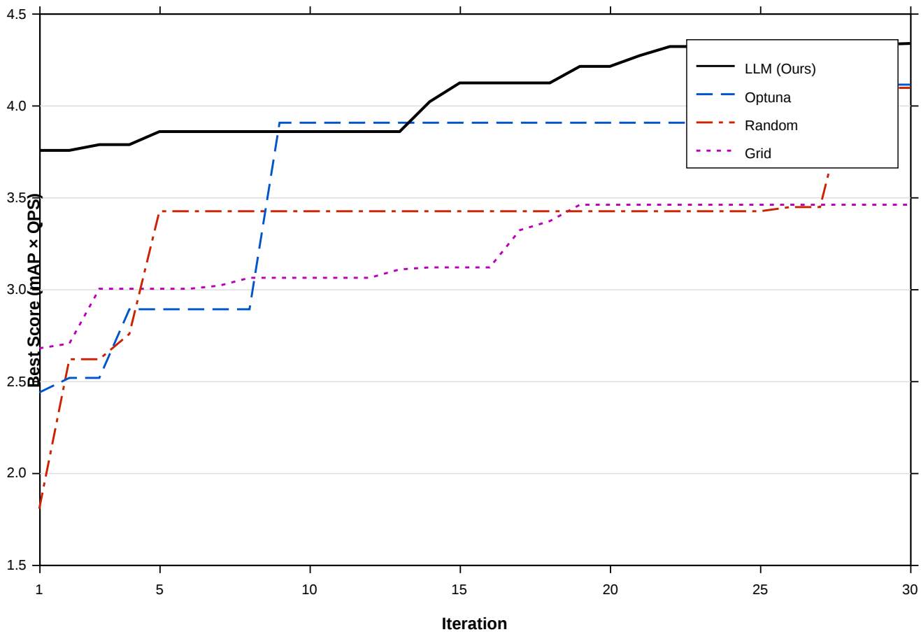
Convergence of Optimization Methods on HICO-DET
