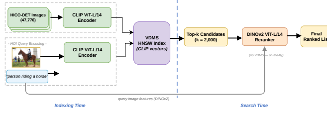
Figure 1: Two-stage retrieval pipeline (oracle O(\theta) ). Stage 1: CLIP ViT-L/14 ANN retrieval produces a top- k candidate pool. Stage 2: DINOv2 ViT-L/14-reg4 distances are fused via convex combination s_j = (1-\alpha)\hat{c}_j + \alpha\hat{d}_j , re-ranking candidates at zero additional indexing cost. Score = mAP \times QPS.
