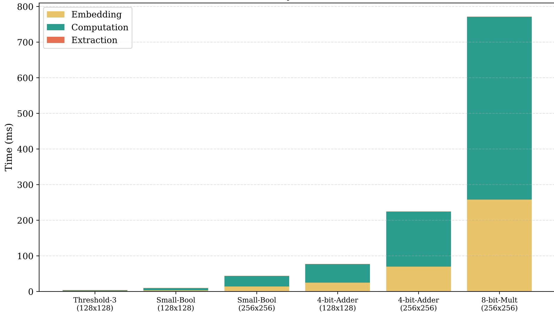
PD-FHC Latency Breakdown (L=4)
