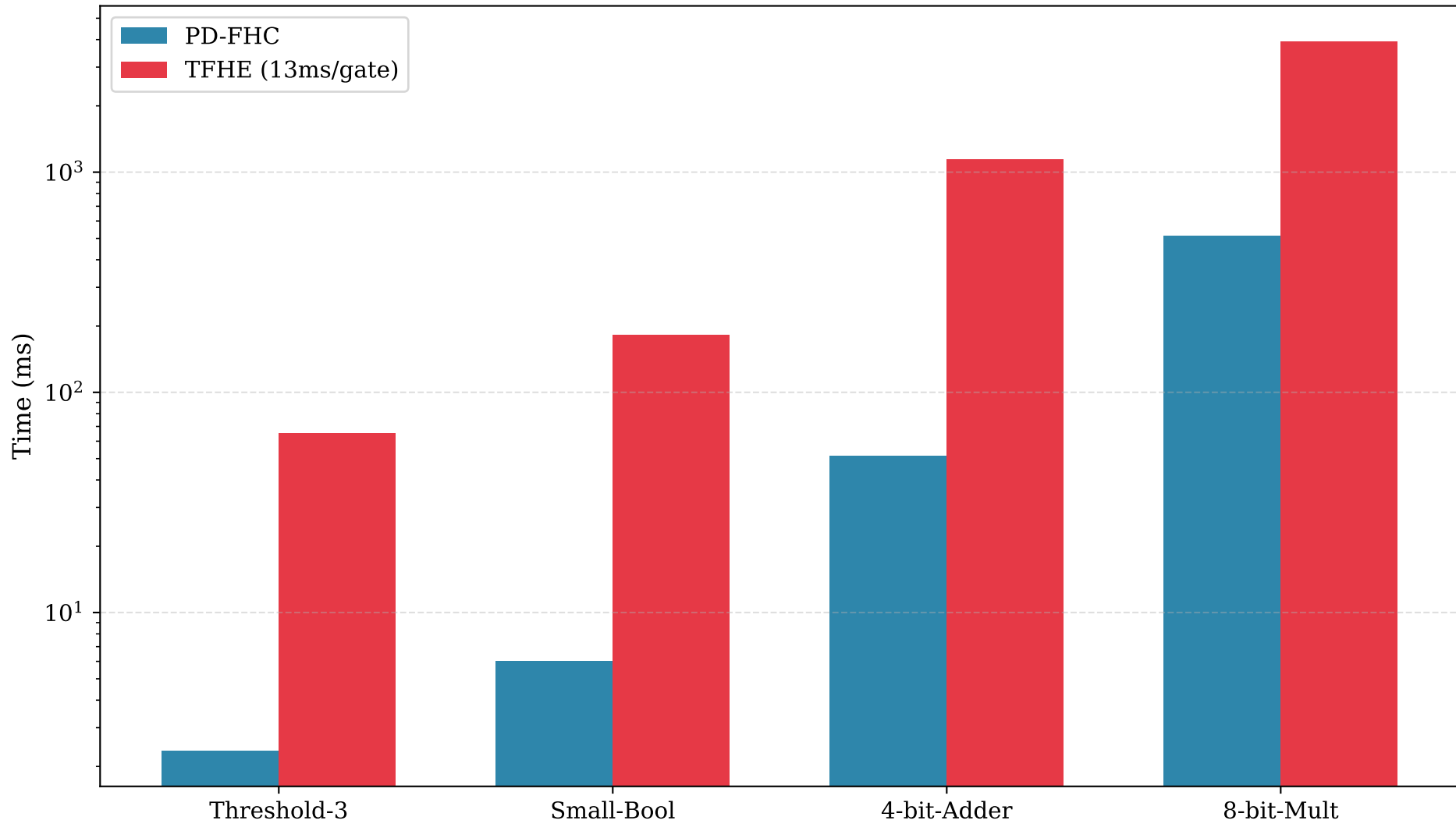
PD-FHC vs TFHE: Boolean Circuit Evaluation
