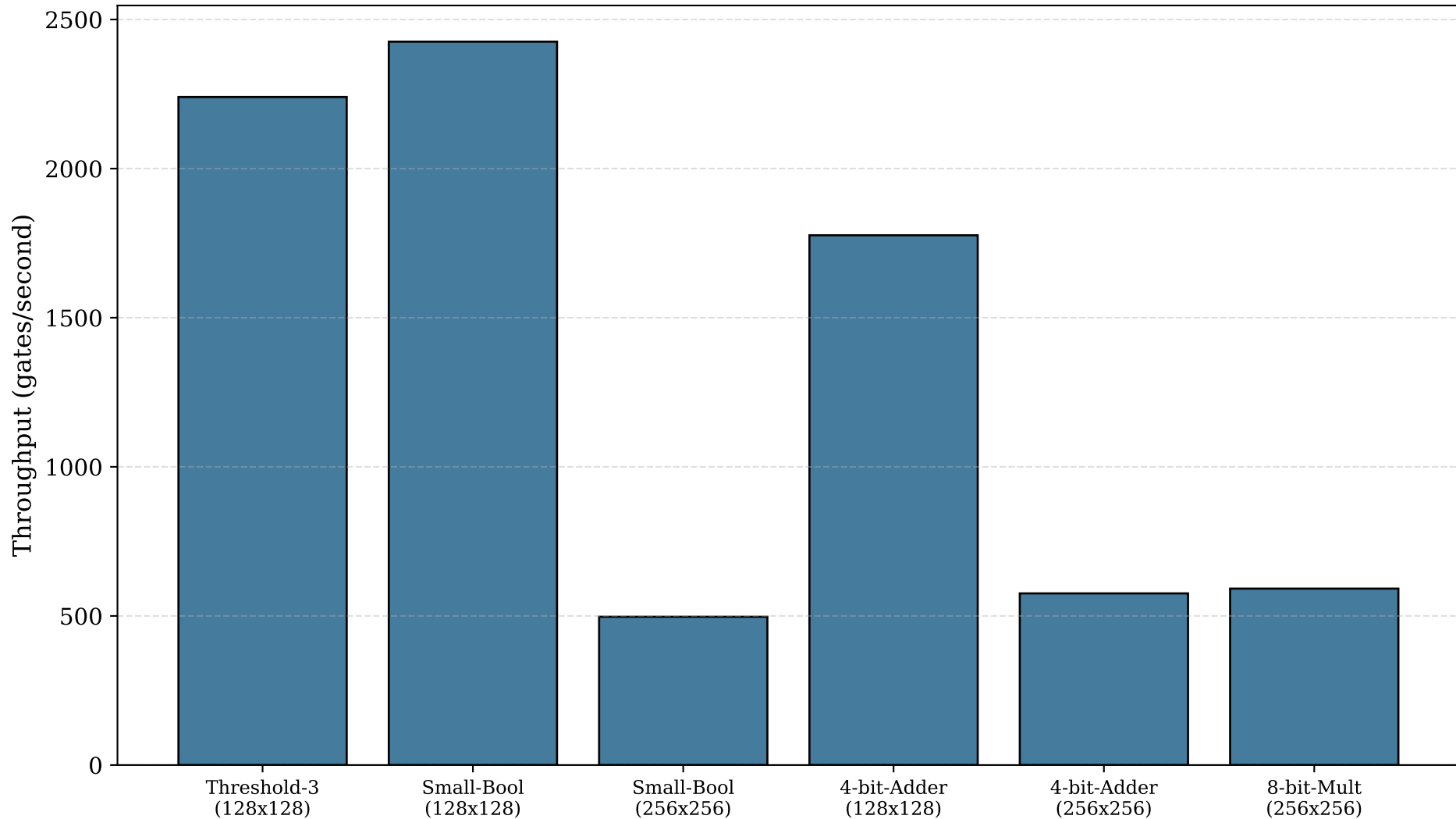
PD-FHC Throughput (L=4)
