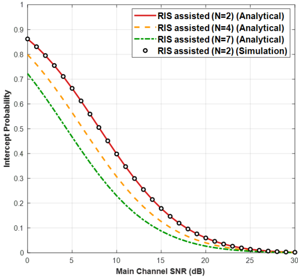
Fig. 2. Effect of N on IP for N_d = 2 , N_e = 2 , and \bar{\gamma}_e = 3 dB.
