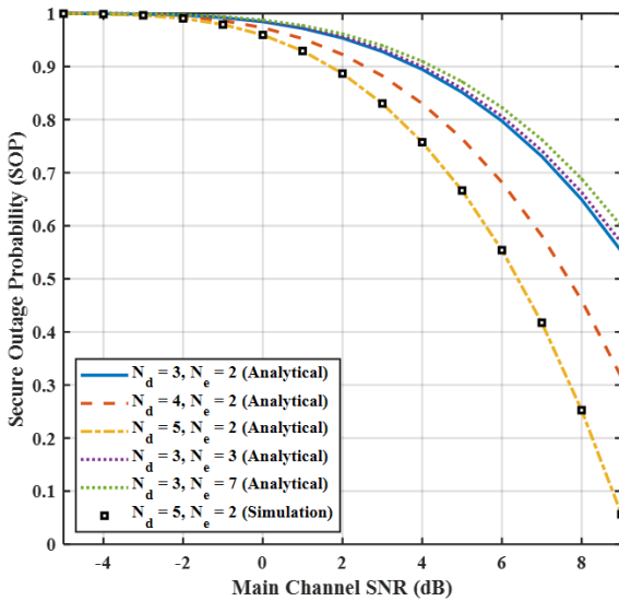
Fig. 6. Variation of SOP with respect to N_d and N_e for N = 4 and \bar{\gamma}_e = 3 dB.
