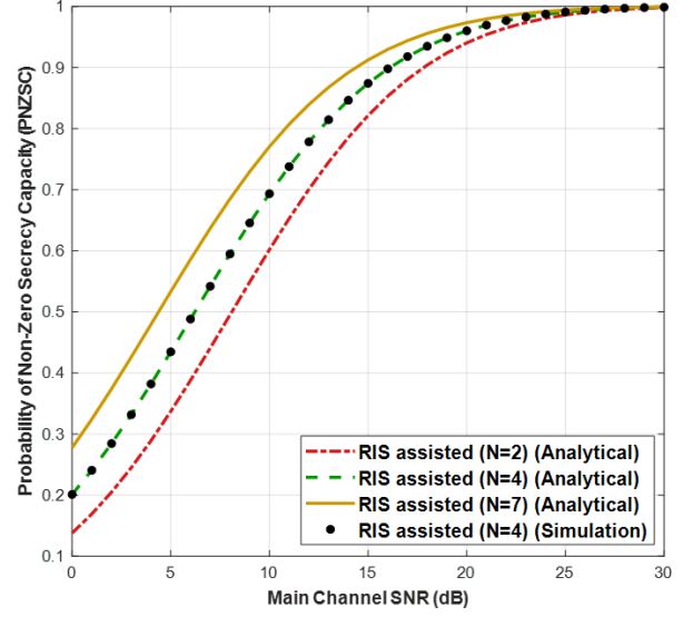
Fig. 3. Impact of N on PNZSC for N_d = 2 , N_e = 2 , and \bar{\gamma}_e = 3 dB.
