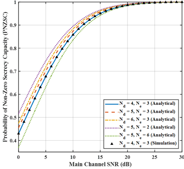
Fig. 5. Variation of PNZSC with respect to N_d and N_e for N = 4 and \bar{\gamma}_e = 3 dB.
