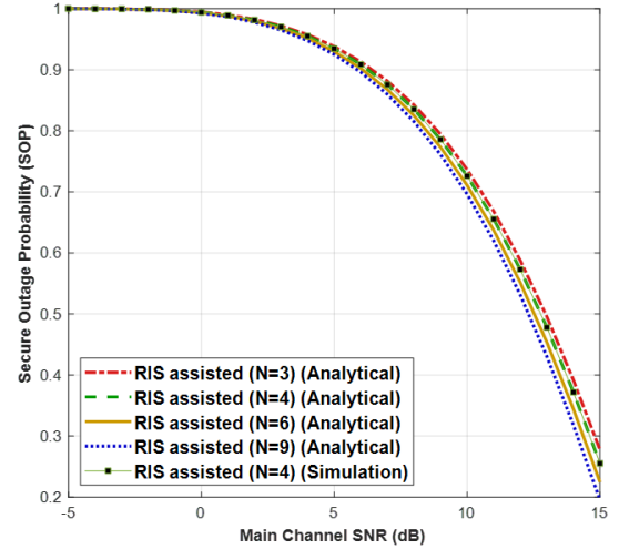
Fig. 4. Impact of N on SOP for N_d = 2 , N_e = 2 , and \bar{\gamma}_e = 3 dB.
