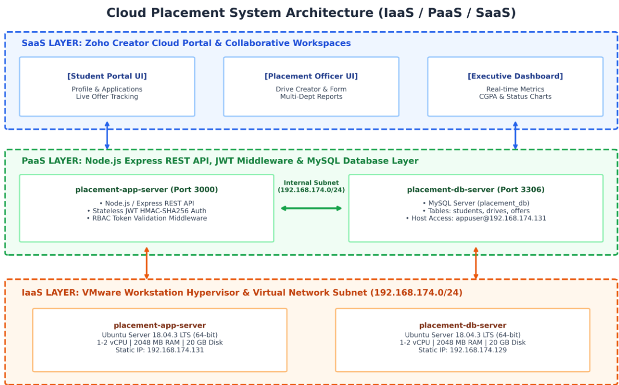
Figure 1: End-to-End Cloud System Architecture and Service Model Mapping (IaaS / PaaS / SaaS)
