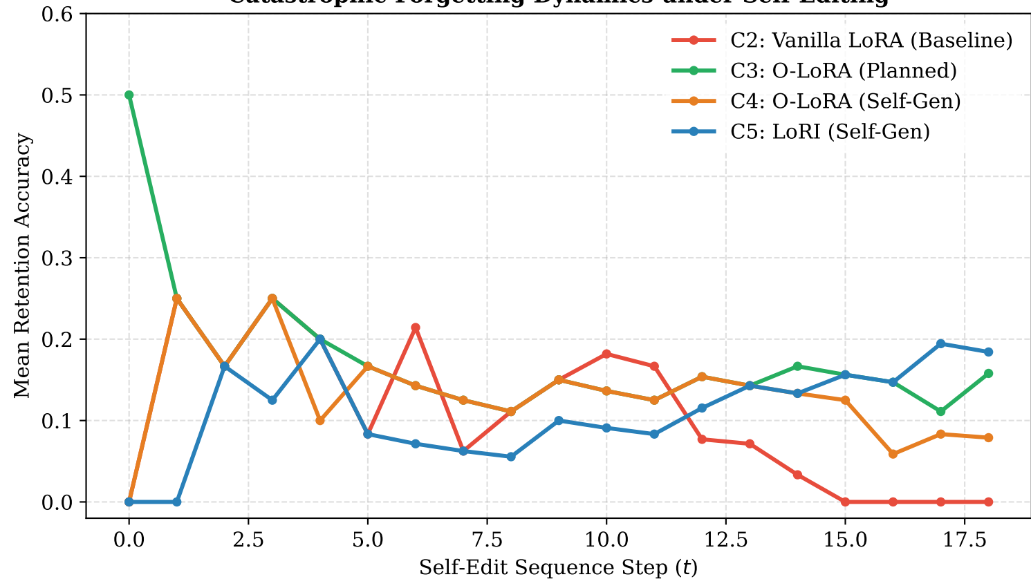
Catastrophic Forgetting Dynamics under Self-Editing
