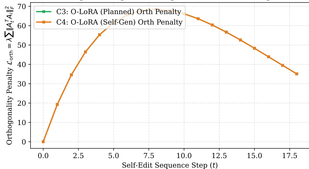
Adapter Subspace Overlap Evolution Across Steps
