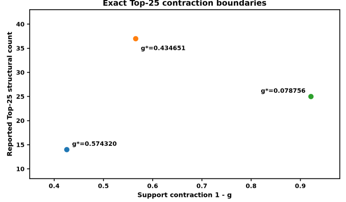
Fig. 2. Three reported exact Top-25 contraction boundaries. All annotations are bold and kept inside the four-sided plotting frame. The post-contraction state is interpreted according to the tie convention in the text.
