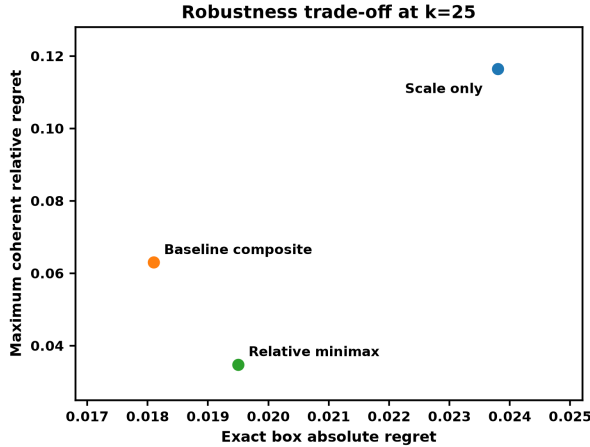
Fig. 3. Robustness trade-off at k = 25 . Labels, tick values, and axes are bold and fully contained within a four-sided frame. Lower is better on both axes; baseline and relative-minimax lists are non-dominating across uncertainty structures.
