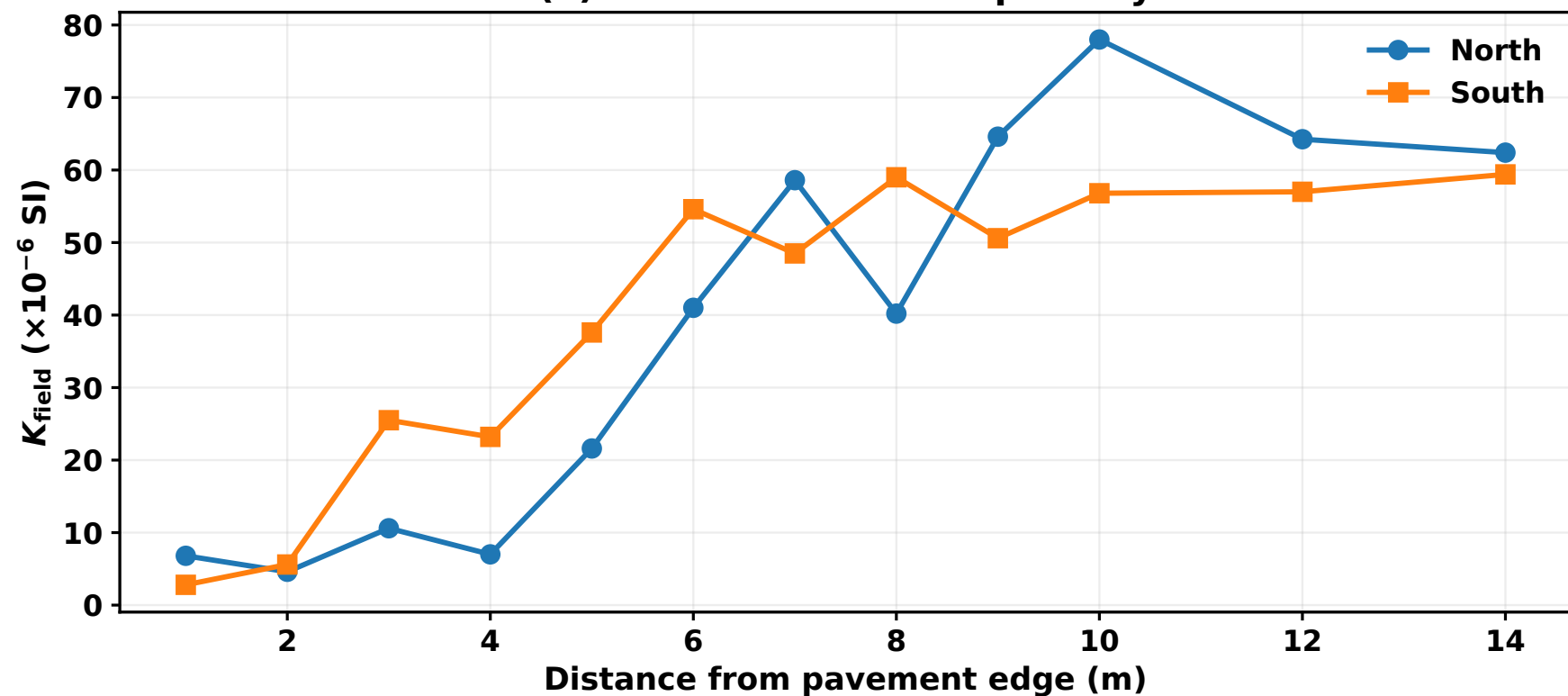
(a) Field volume susceptibility
