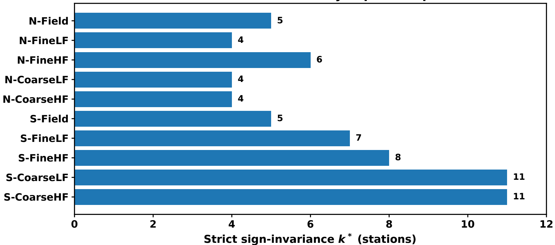
(b) Direction recoverability is profile-specific
