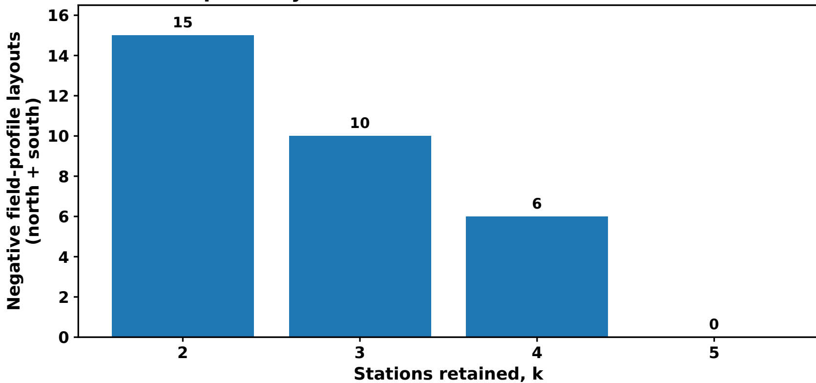
(a) Sparse layouts can reverse the observed direction
