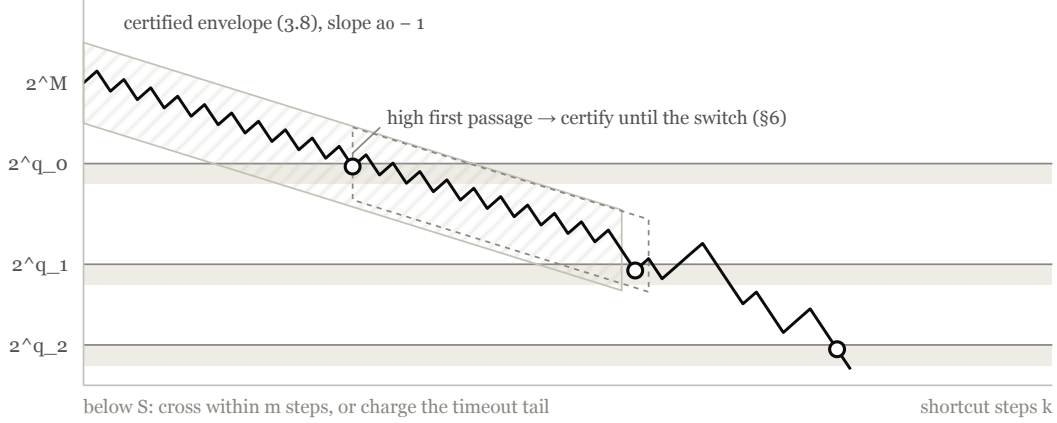
(a) high certification and timeout continuation — a real orbit in I_M , M = 40 orbit value
