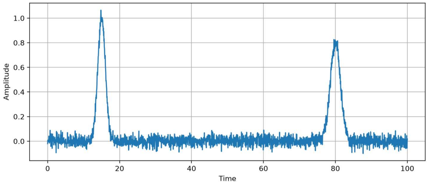
Ultrasonic A-Scan — Normal
