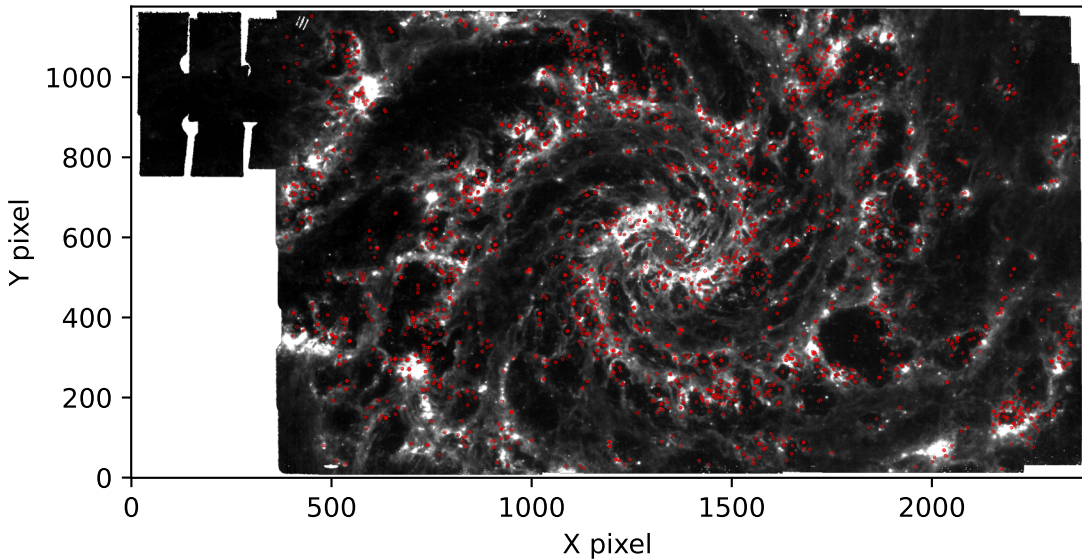
Bubble Positions on JWST F770W Image
