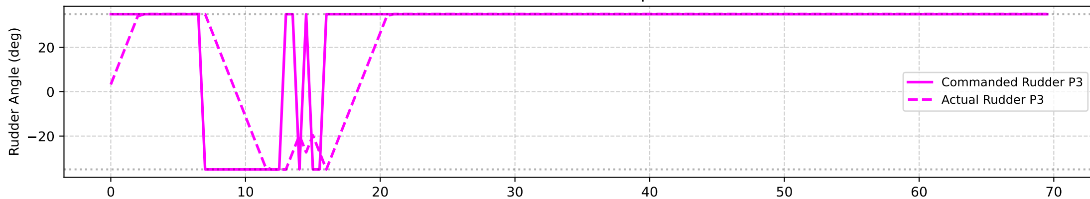
Evader Rudder Response
