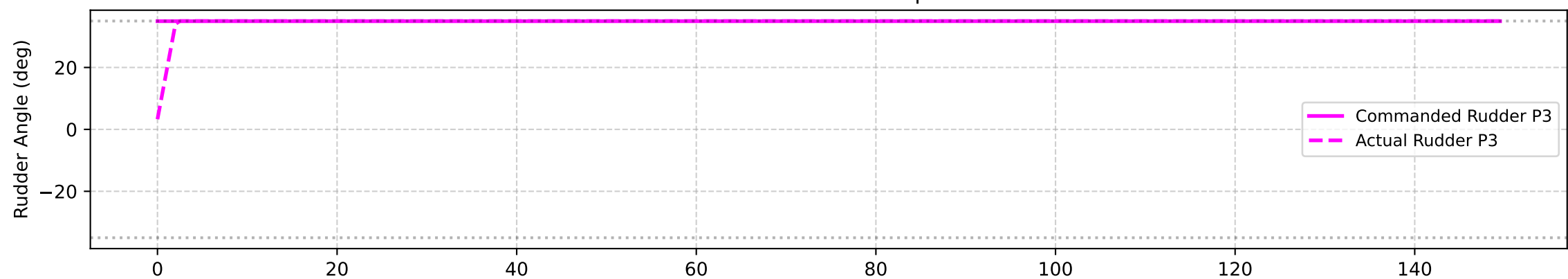
Evader Rudder Response
