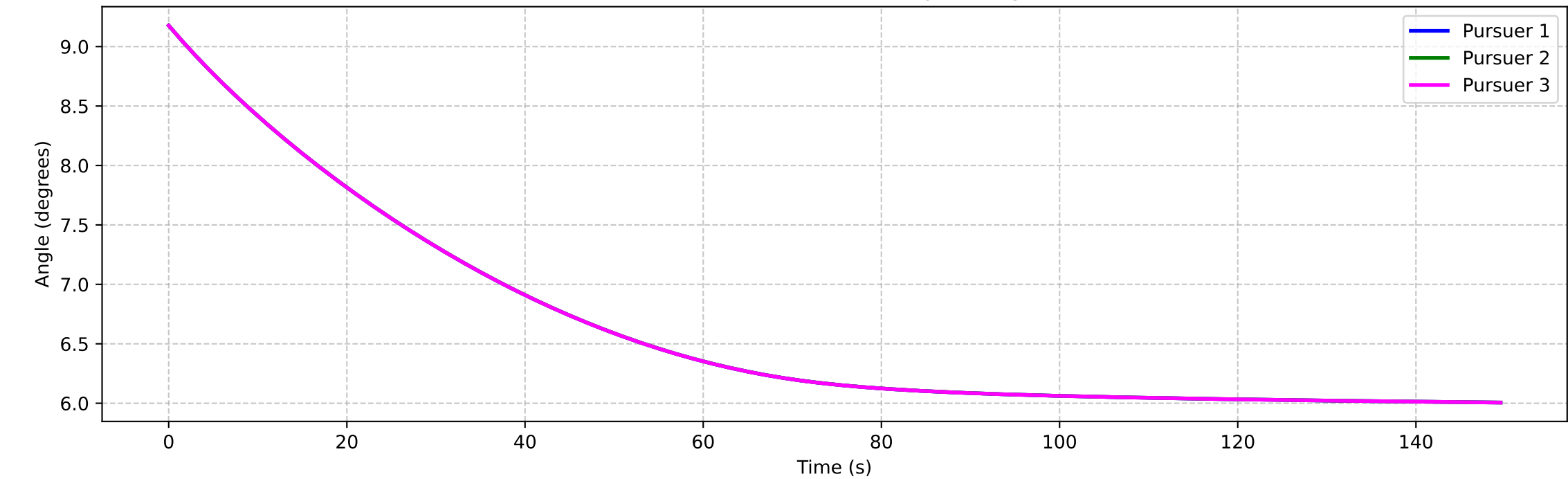
Evolution of Individual Occupied Angles
