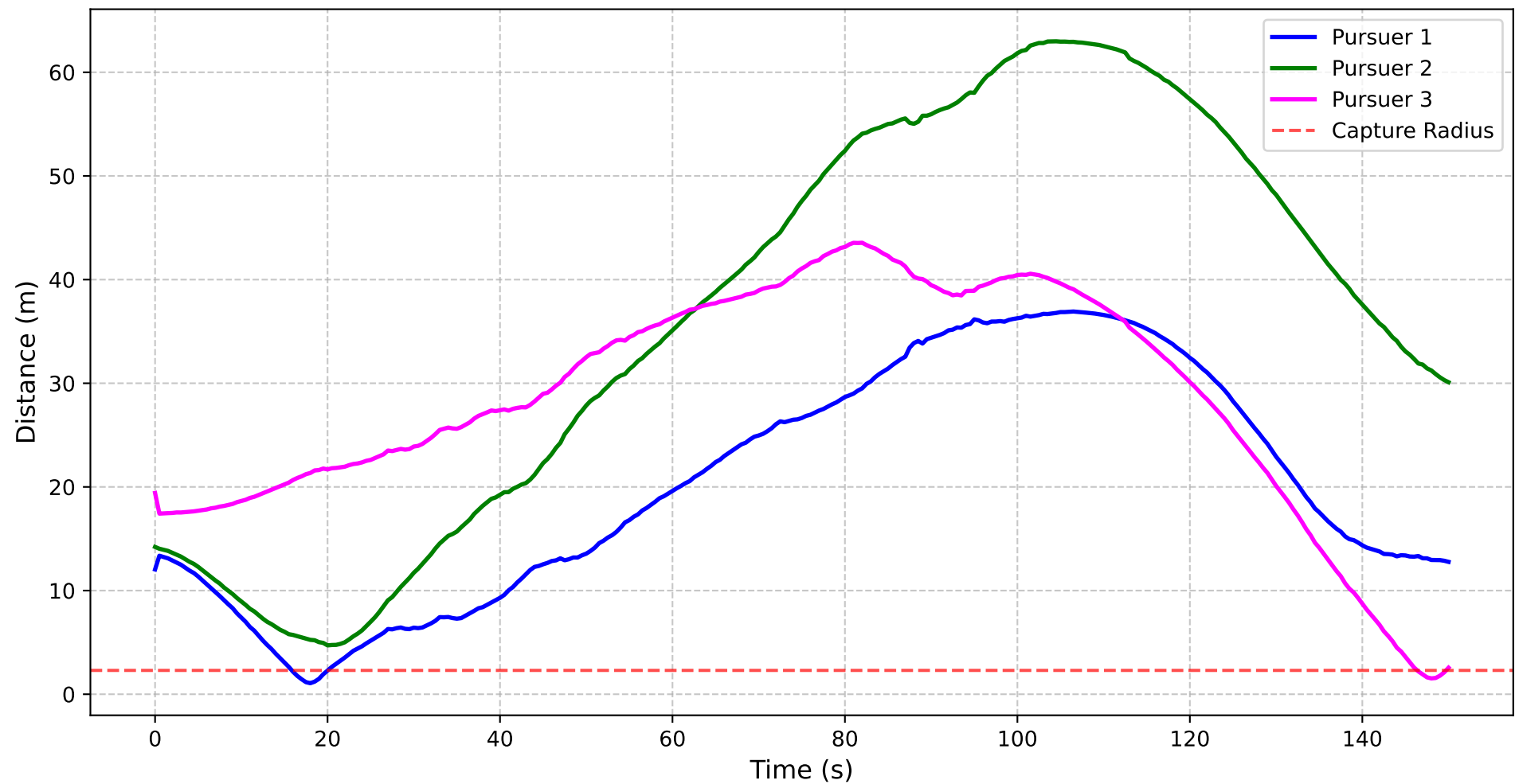
Distance between Pursuers and Evader
