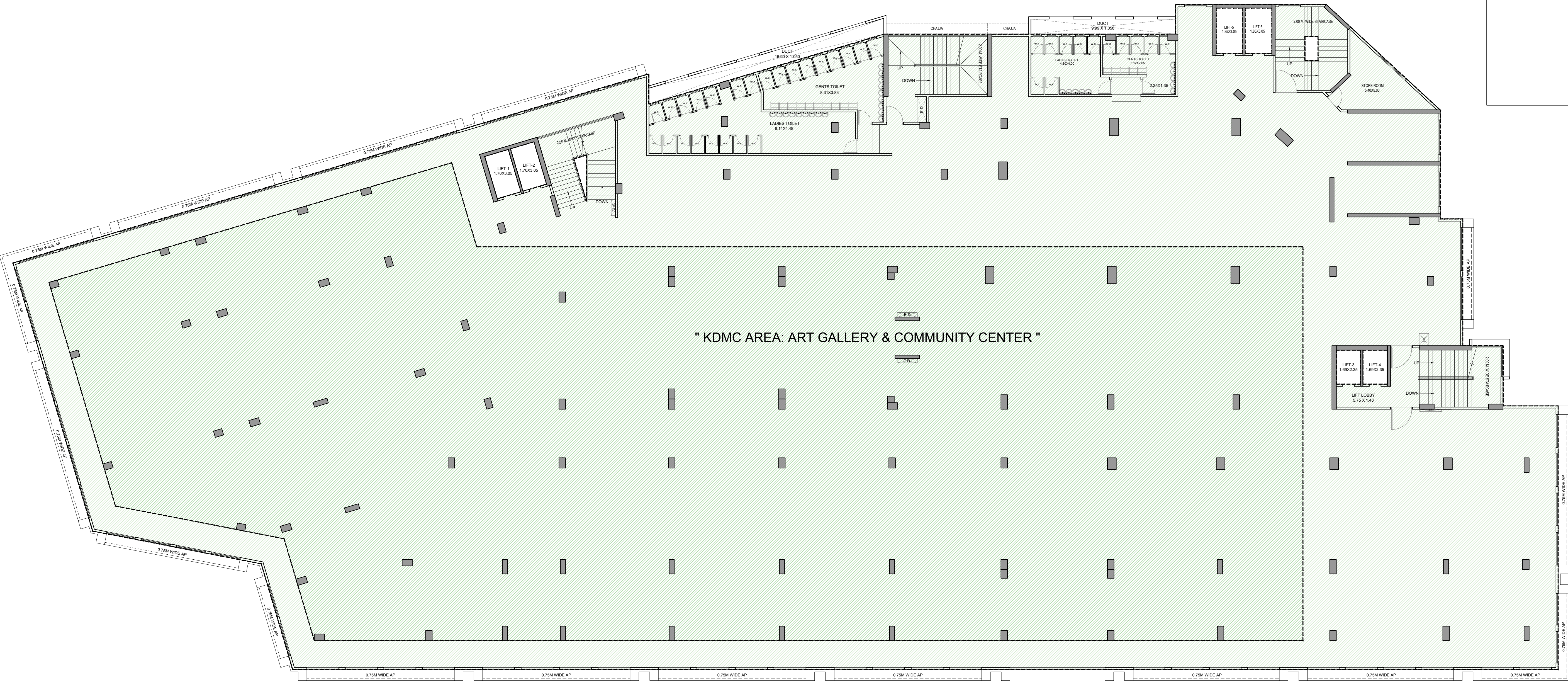
2ND & 3RD FLOOR PLAN
