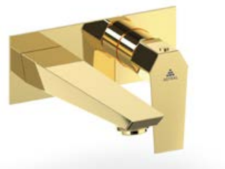
AF720116GLBR Exposed Part of Wall Mounted Basin Cock with Spout and Operating Lever with 2 mm Thick Solid Flange MRP: 6700 Suitable for Concealed Body AF900911CHBR MRP: 1825
