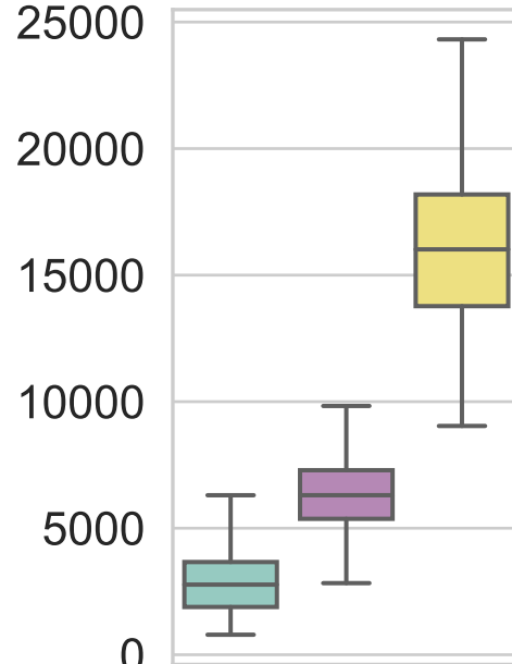
LIX
