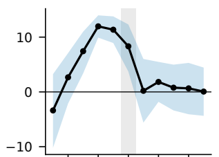
(k) Downward solar ( \text{W m}^{-2} )
