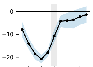
(j) Downward longwave ( \text{W m}^{-2} )
