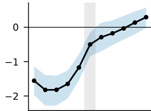
(f) T850, BD (K)
