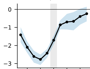
(i) 2-m dewpoint, BD ( ^{\circ}\text{C} )
