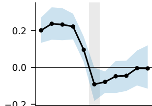
(h) Z500, South Asia (m)
