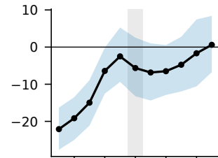
(h) Z500, South Asia (m)
