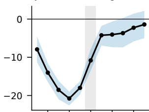
(j) Downward longwave ( \text{W m}^{-2} )
