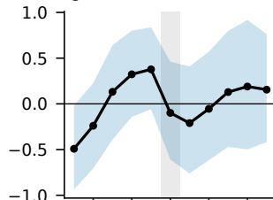
(g) MSLP, BD (hPa)
