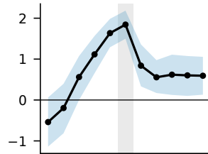
(g) MSLP, BD (hPa)
