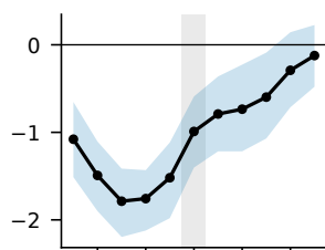
(f) T850, BD (K)
