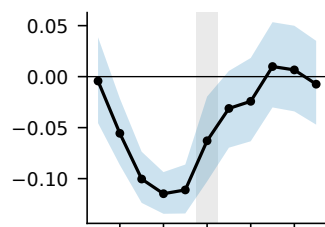
(l) Total cloud (fraction)
