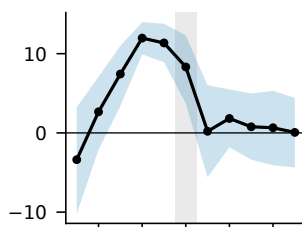
(k) Downward solar ( \text{W m}^{-2} )
