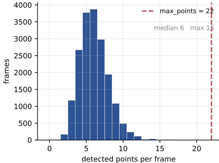
Point-count distribution
