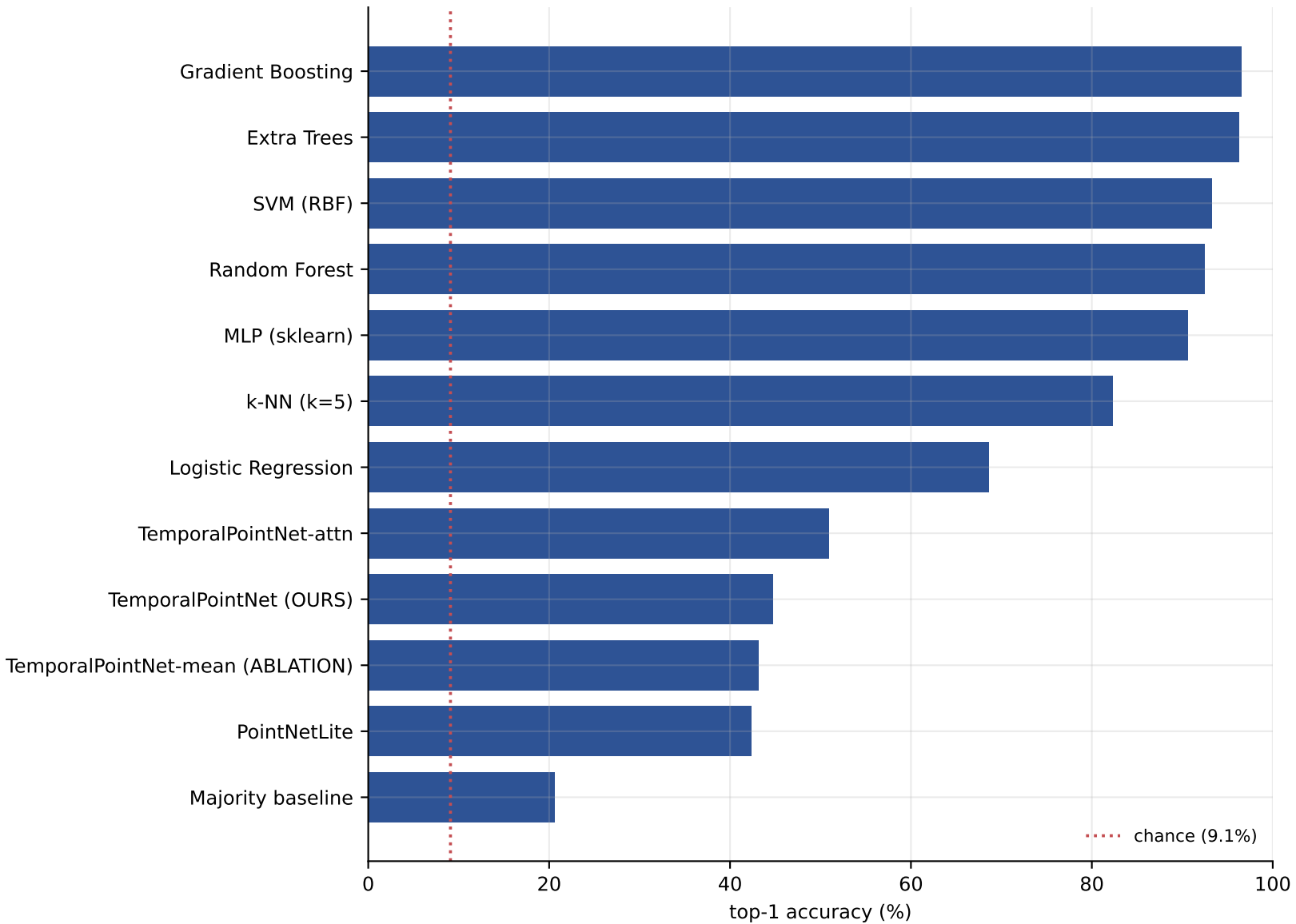
Identification accuracy — all models
