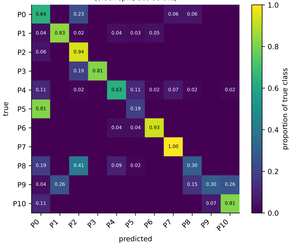
Confusion matrix — TemporalPointNet-attn (block split, acc 68.6%)
