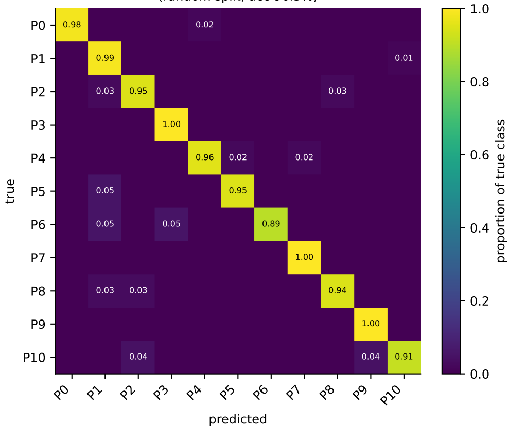
(random split, acc 96.5%)
