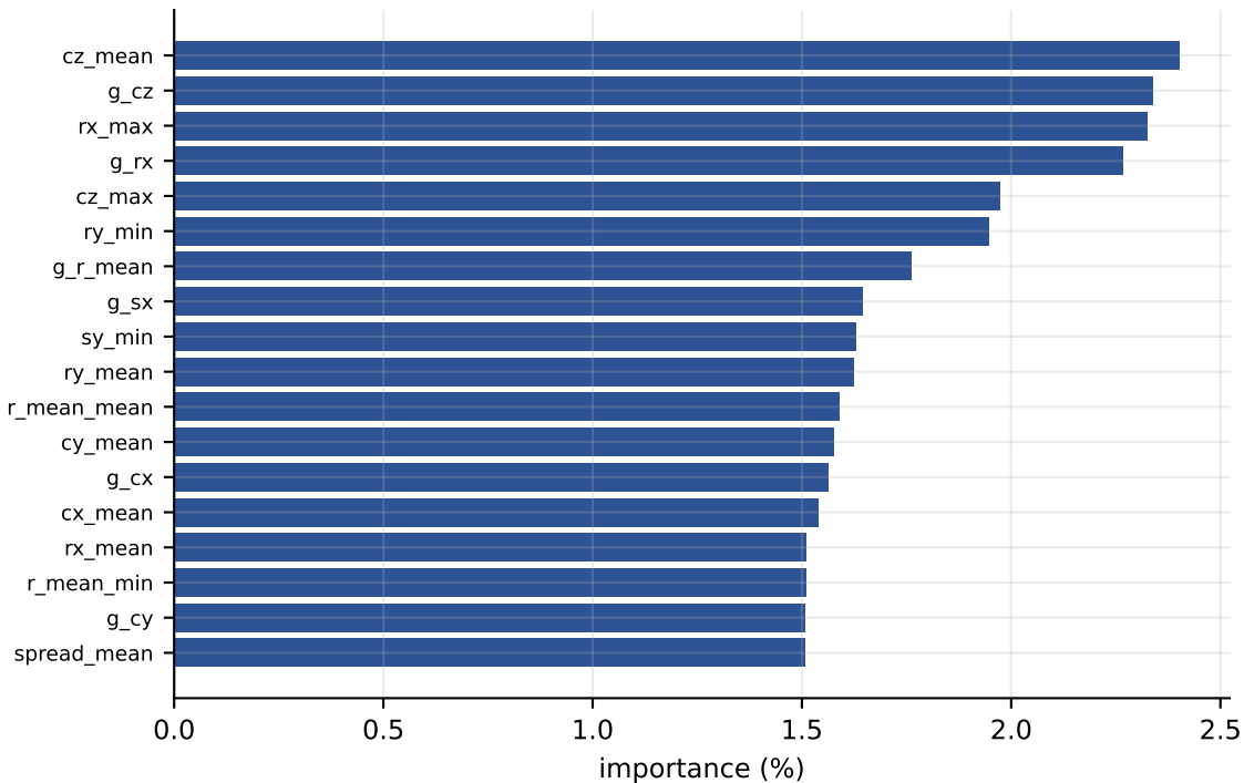
Most informative handcrafted features
