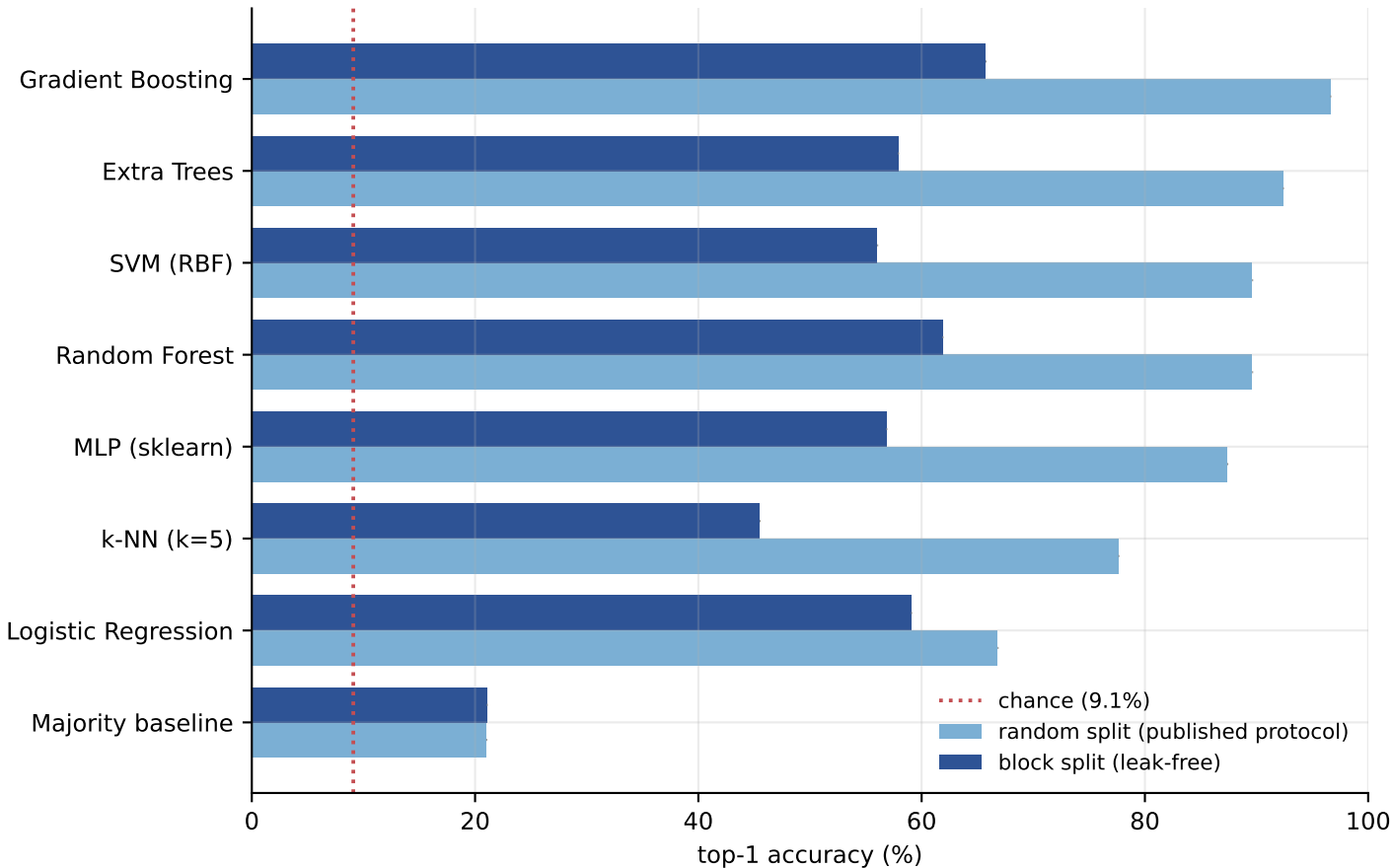
Identification accuracy — all models
