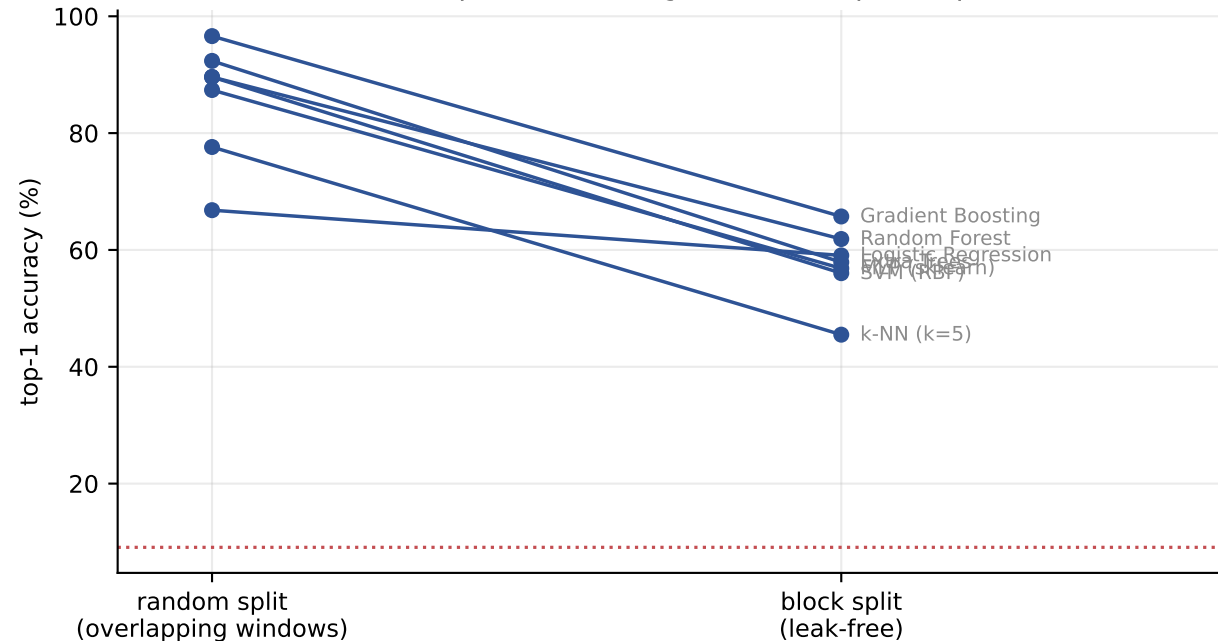
Evaluation-protocol leakage: mean drop 28.2 points
