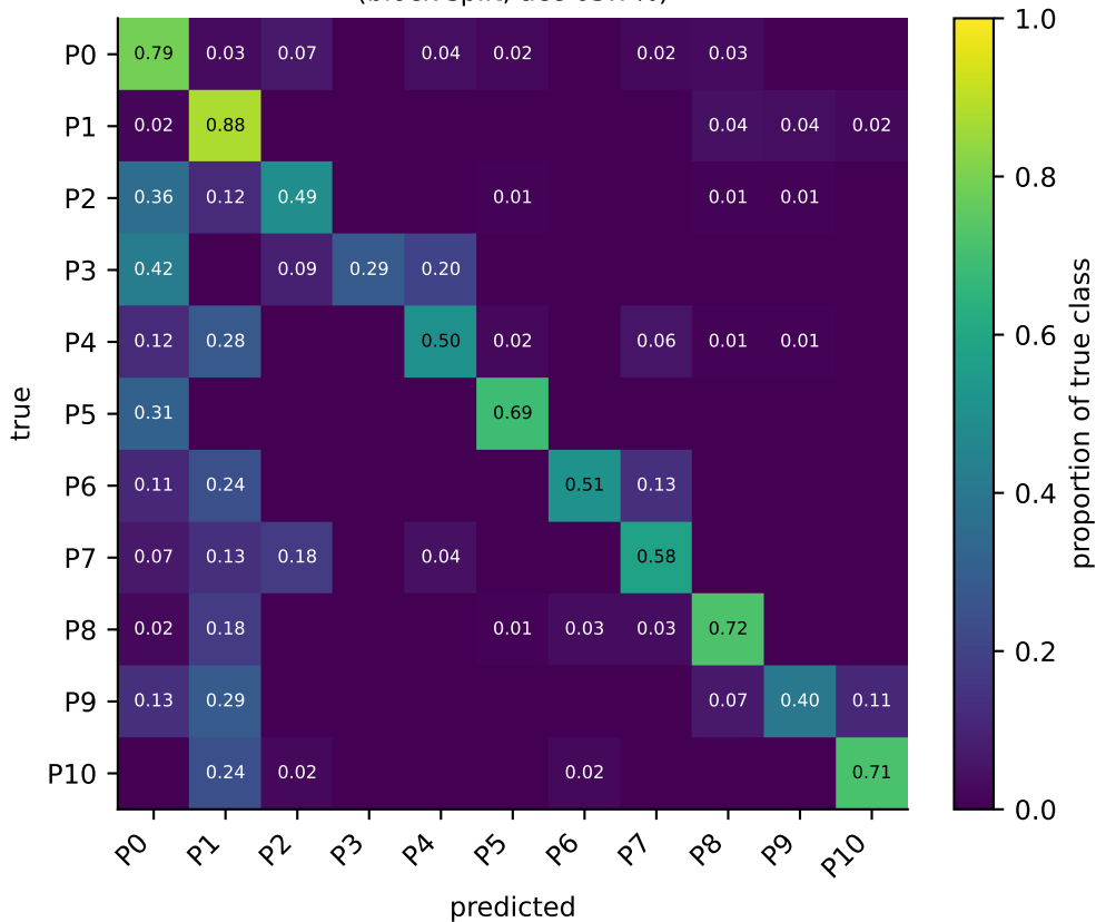
Confusion matrix — Gradient Boosting (block split, acc 65.7%)
